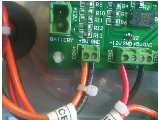
5 volt power wires to be removed ( Orange and Black connected to Con4)
