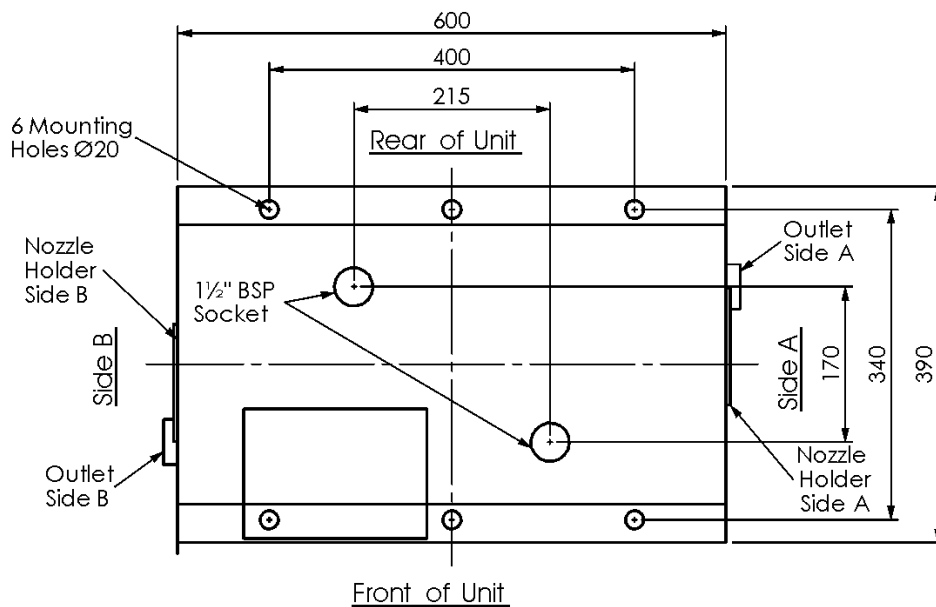
Footprint Plan View
