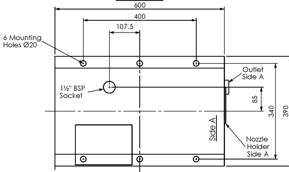
Footprint Plan View
